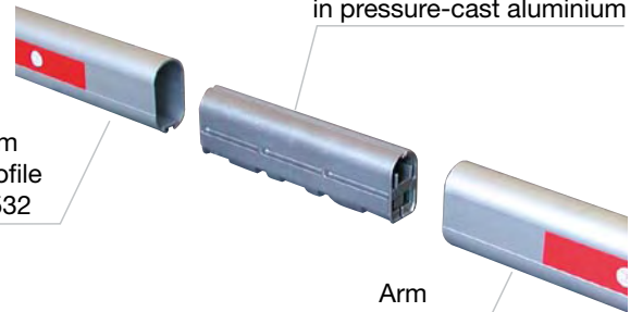
Internal arm joint terminal in pressure-cast aluminium
